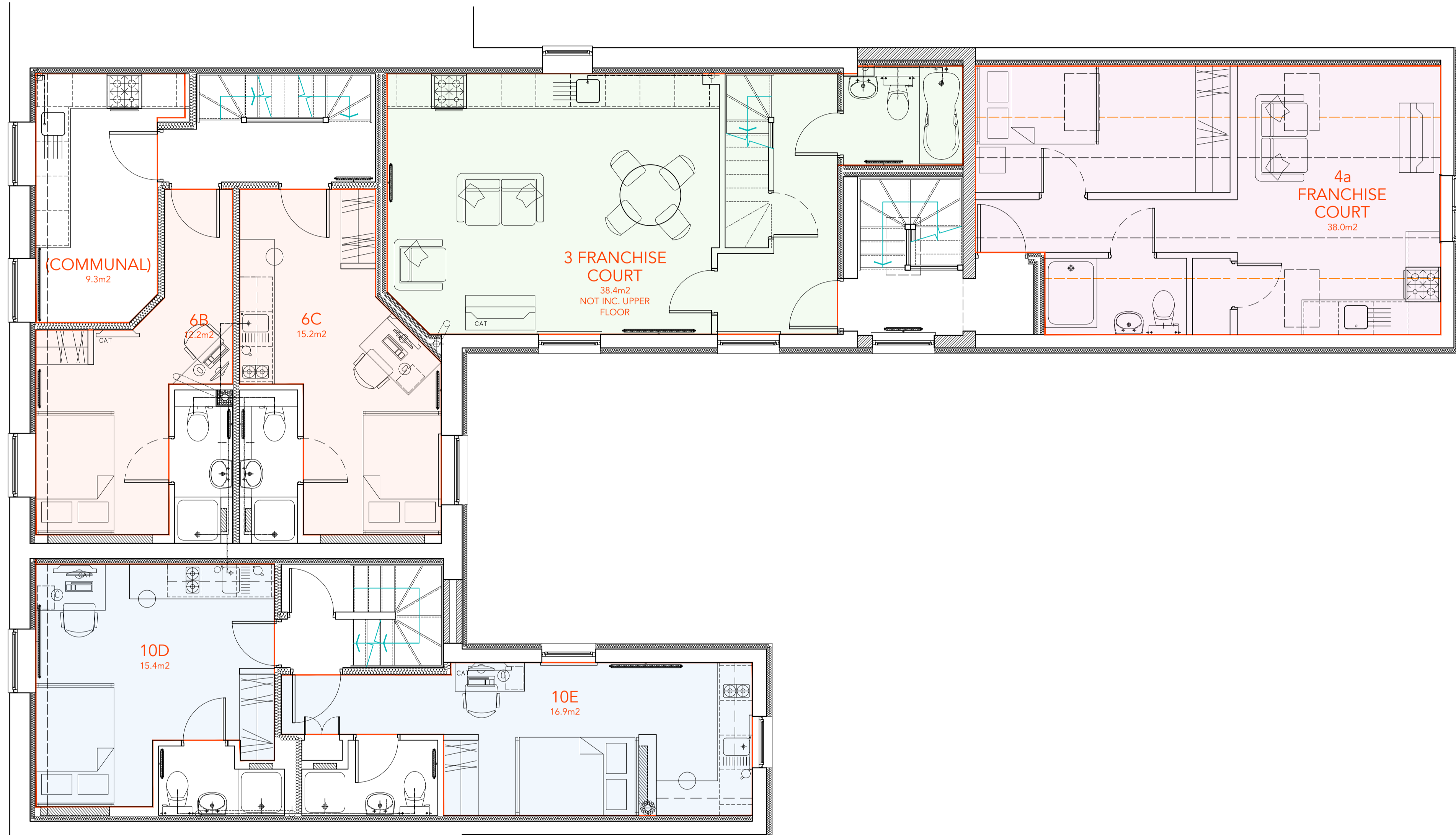
PROPOSED FIRST FLOOR LAYOUT 1:50
